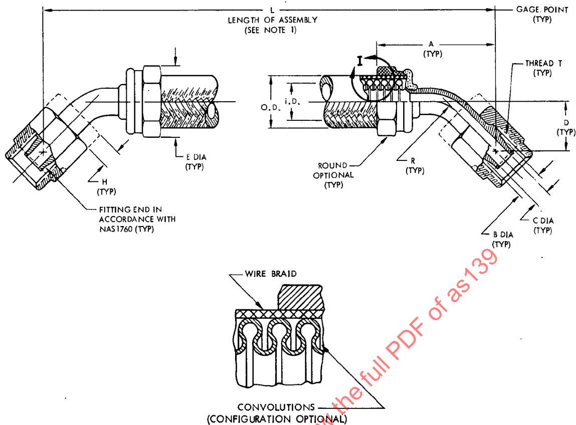
DETAIL I
