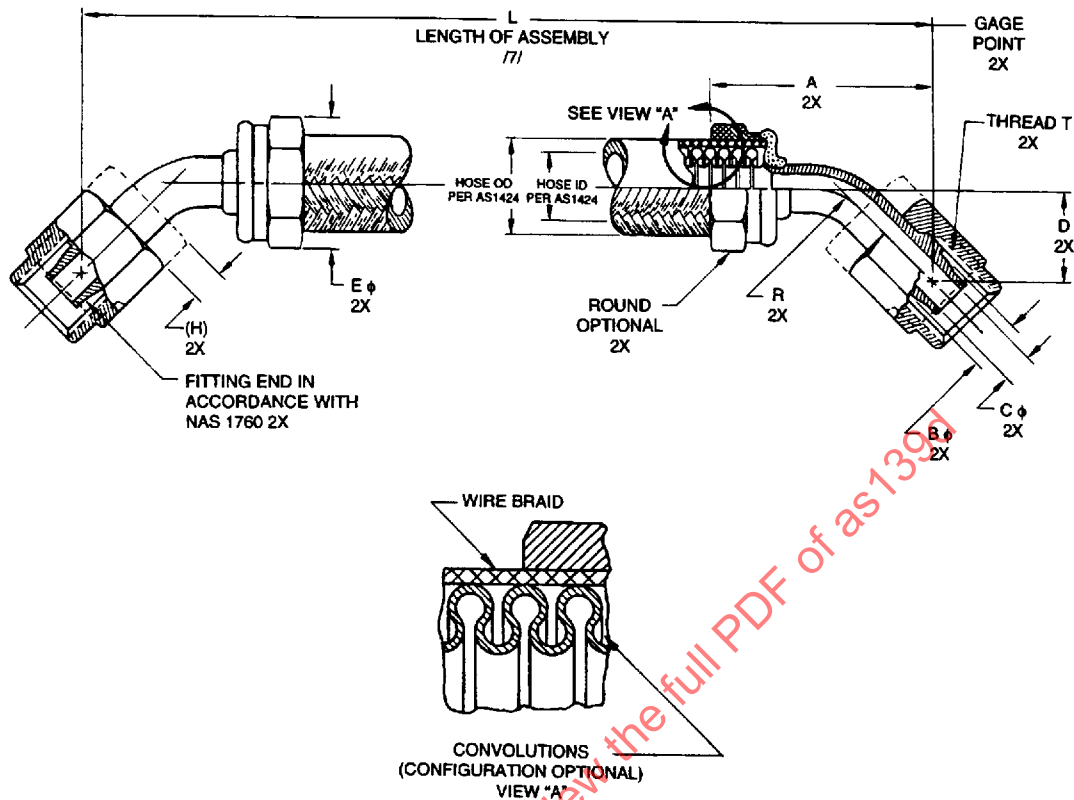
FIGURE 1 - HOSE ASSEMBLY
