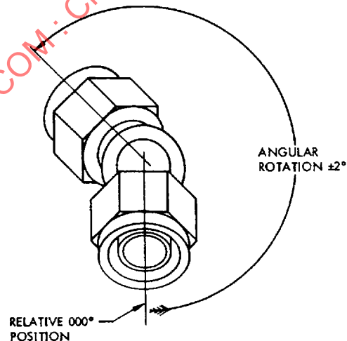
FIGURE 2 - FITTING ANGULAR ORIENTATION /11/
