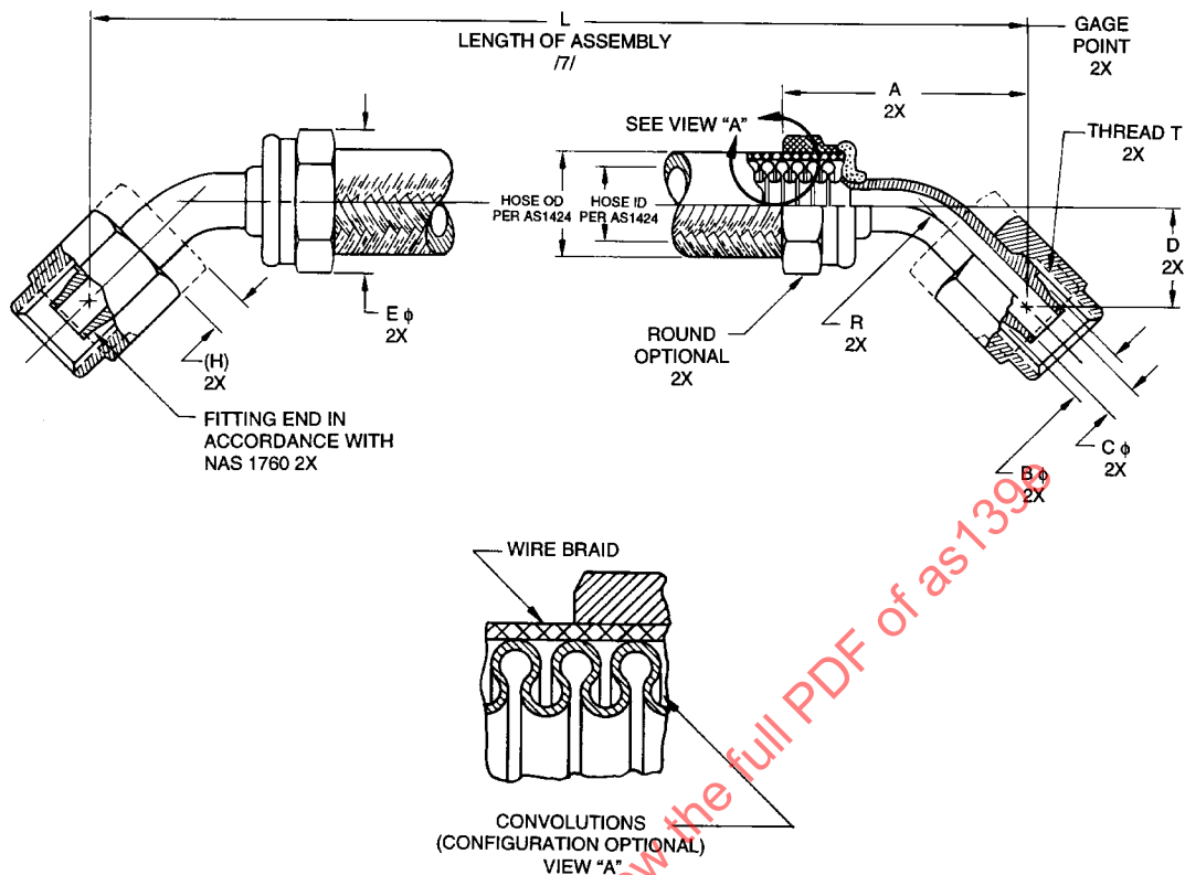
FIGURE 1 - HOSE ASSEMBLY
