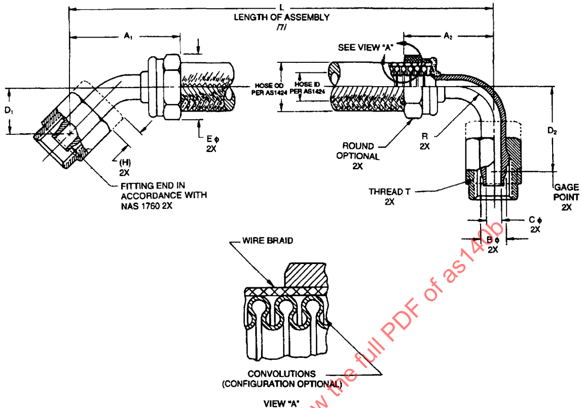
FIGURE 1 - HOSE ASSEMBLY
