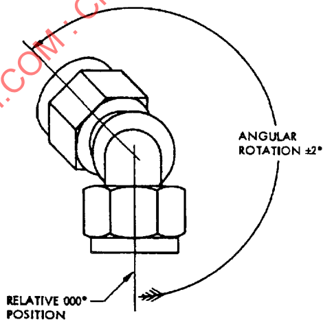
FIGURE 2 - FITTING ANGULAR ORIENTATION /1/
