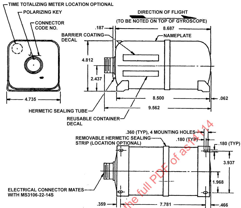
MS14114-2 GYROSCOPE
