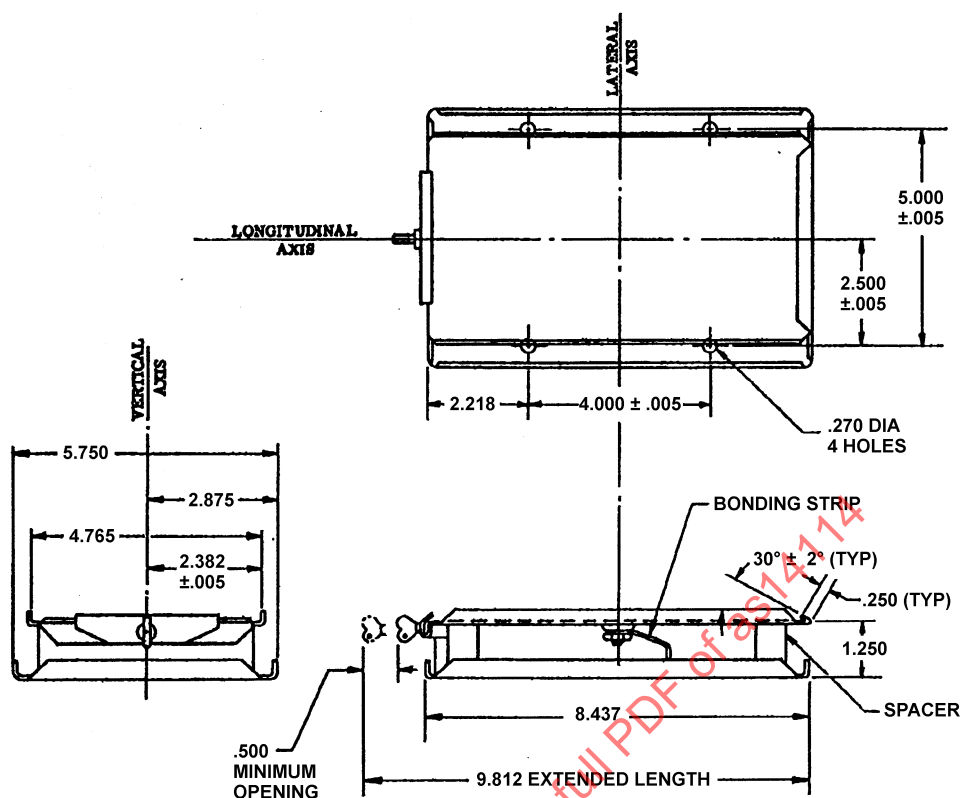
MS14114-3 MOUNT
