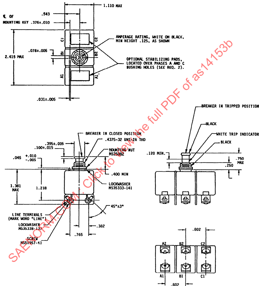
FIGURE 1 - TRIP-FREE CIRCUIT BREAKER
