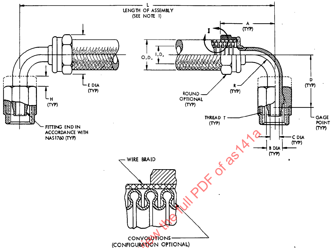
DETAIL I
