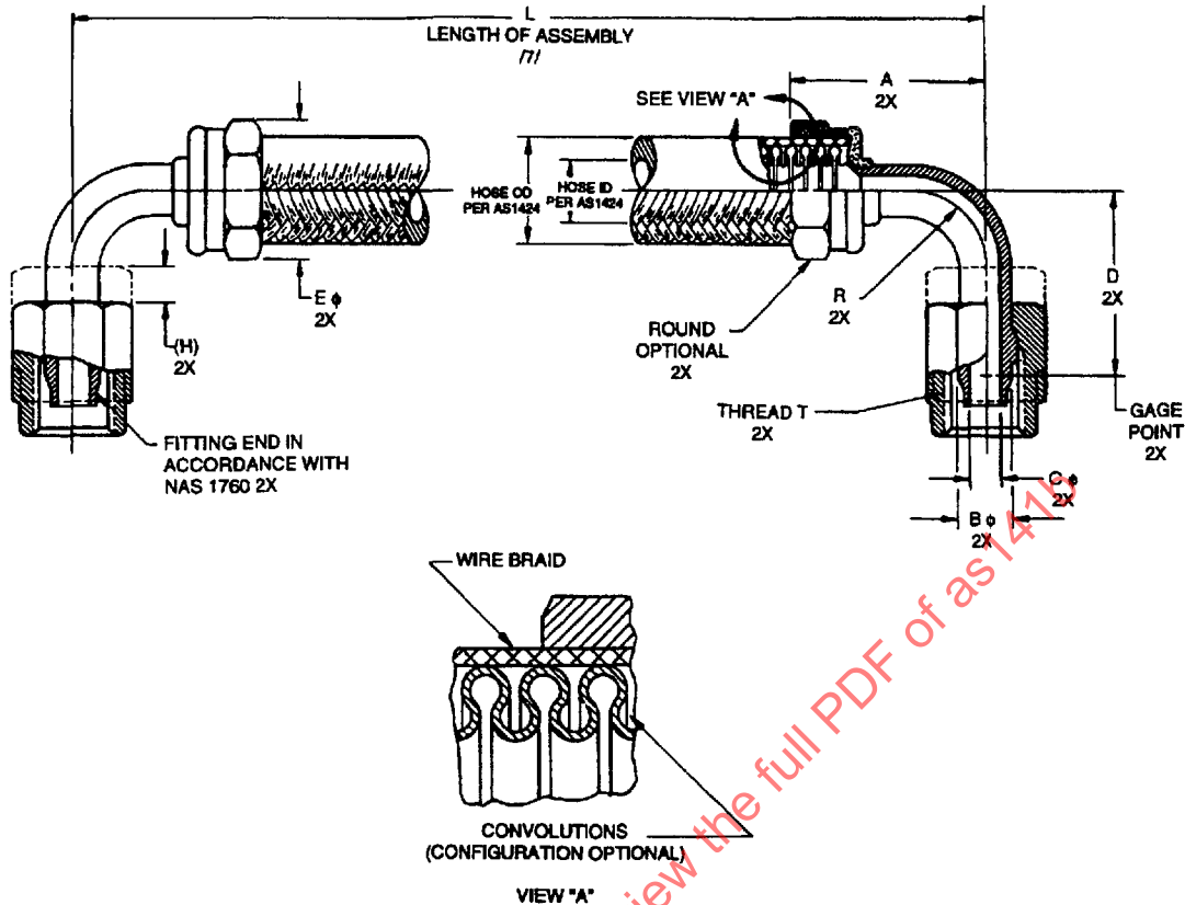
FIGURE 1 - HOSE ASSEMBLY
