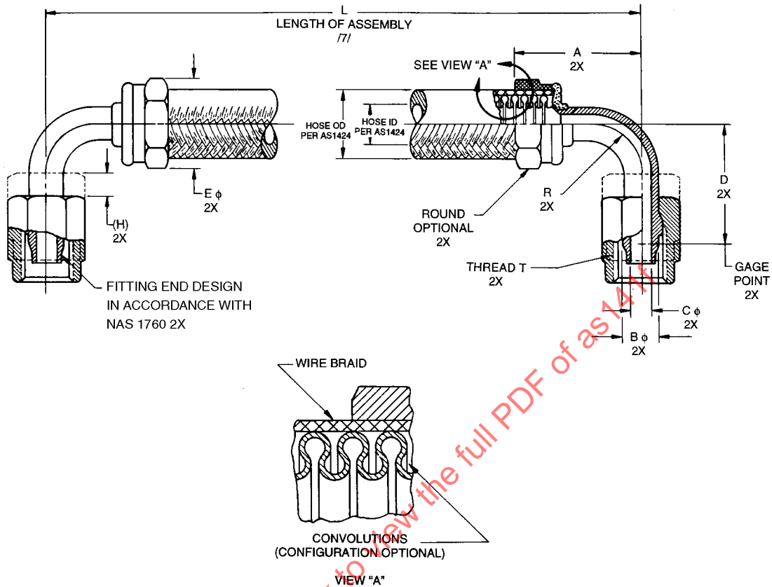
FIGURE 1 - HOSE ASSEMBLY
