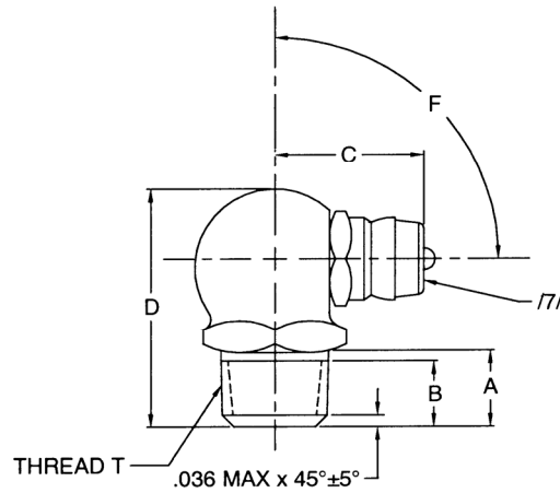
FIGURE 3 - FITTING, ELBOW 90°
