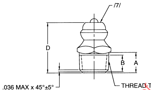
FIGURE 1 - FITTING, STRAIGHT
