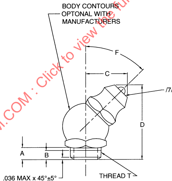
FIGURE 2 - FITTING, ELBOW
