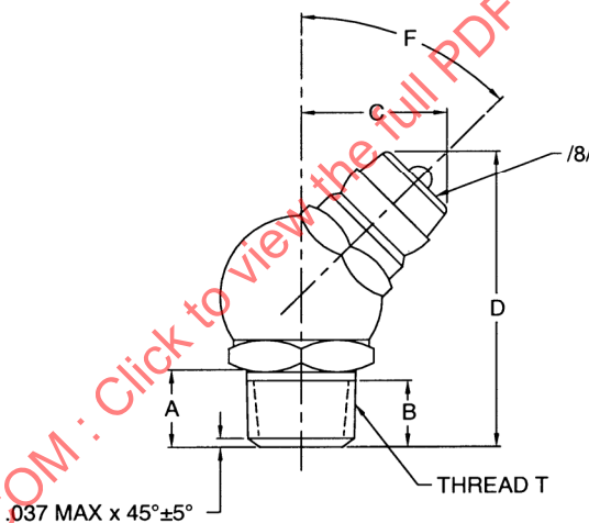
FIGURE 2 - FITTING, ELBOW
