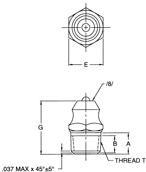
FIGURE 1 - FITTING, STRAIGHT
