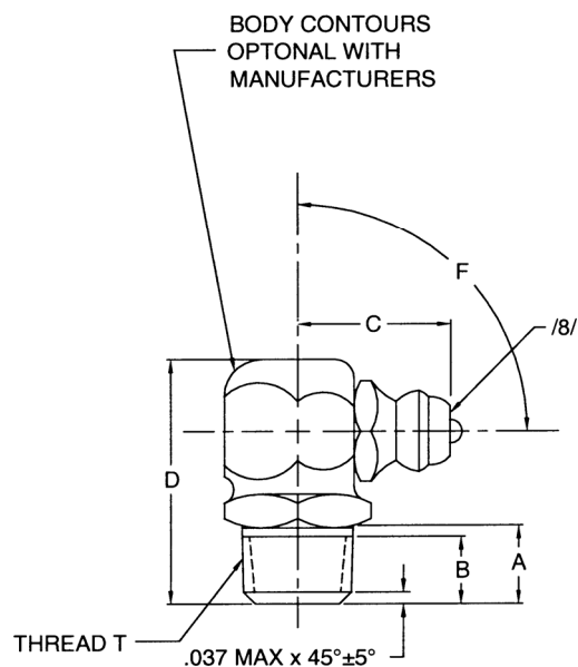
FIGURE 3 - FITTING, ELBOW 90°
