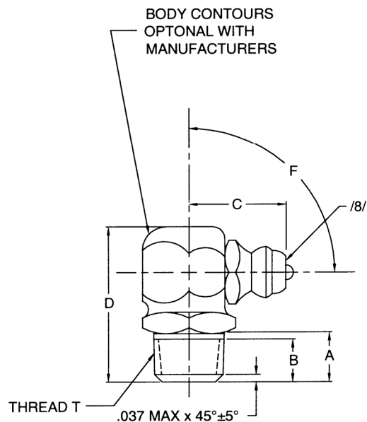
FIGURE 3 - FITTING, ELBOW 90°
