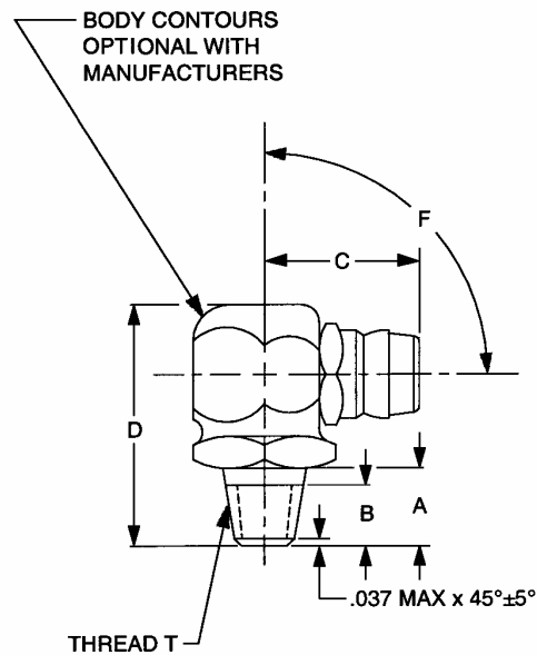
FIGURE 3 - FITTING, ELBOW, 90°
