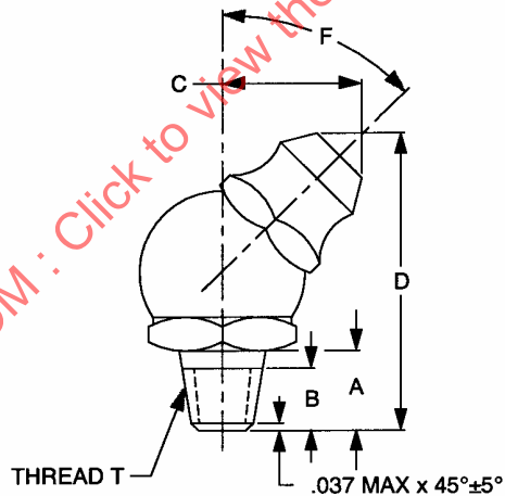
FIGURE 2 - FITTING, ELBOW
