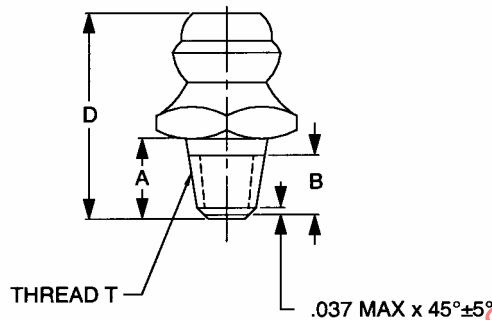
FIGURE 1 - FITTING, STRAIGHT
