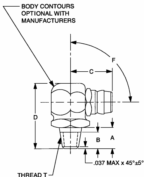
FIGURE 3 - FITTING, ELBOW, 90°
