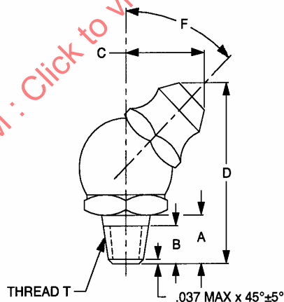
FIGURE 2 - FITTING, ELBOW
