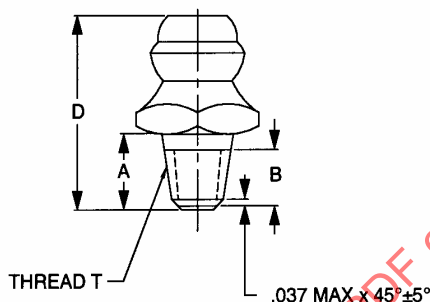
FIGURE 1 - FITTING, STRAIGHT
