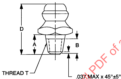
FIGURE 1 - FITTING, STRAIGHT
