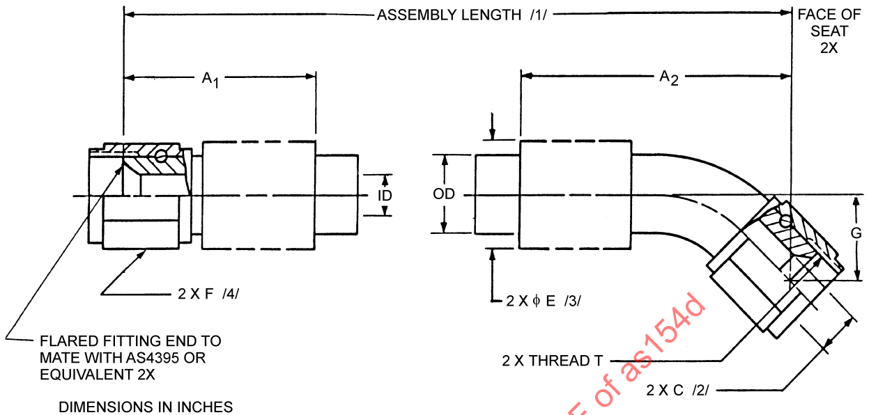
FIGURE 1 - HOSE AND FITTING DIMENSIONS
