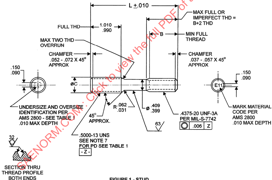
FIGURE 1 - STUD
