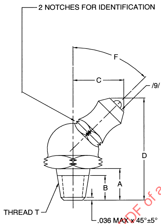
FIGURE 2 - FITTING, ELBOW
