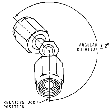
FIGURE 3 - FITTING ANGULAR ORIENTATION
