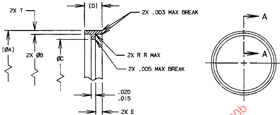
SECTION A-A ENLARGED
