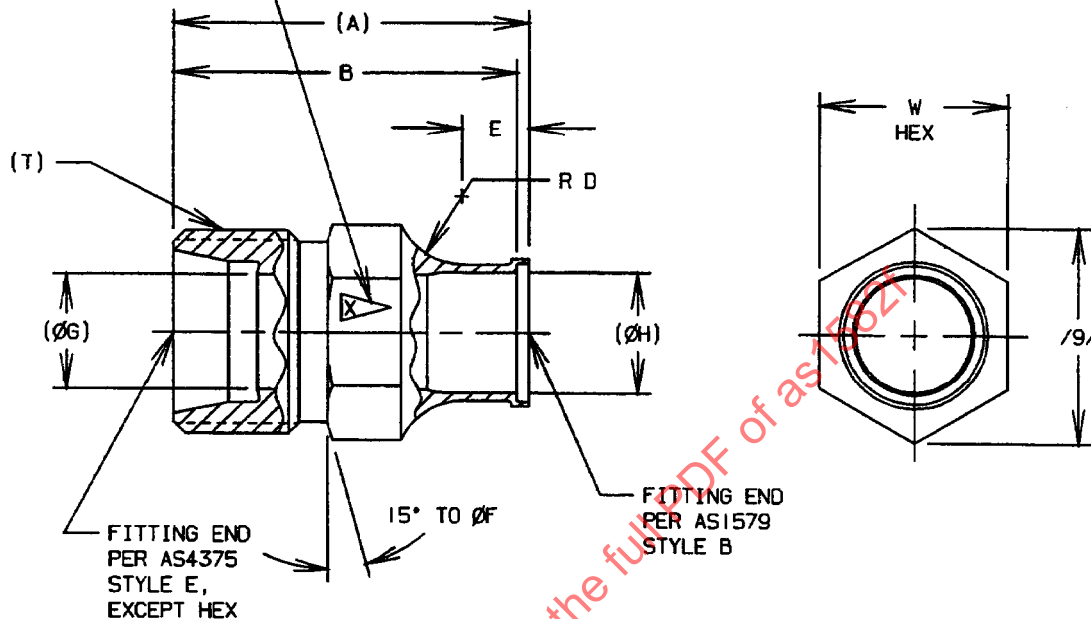
FIGURE 1 - FITTING, ADAPTER
