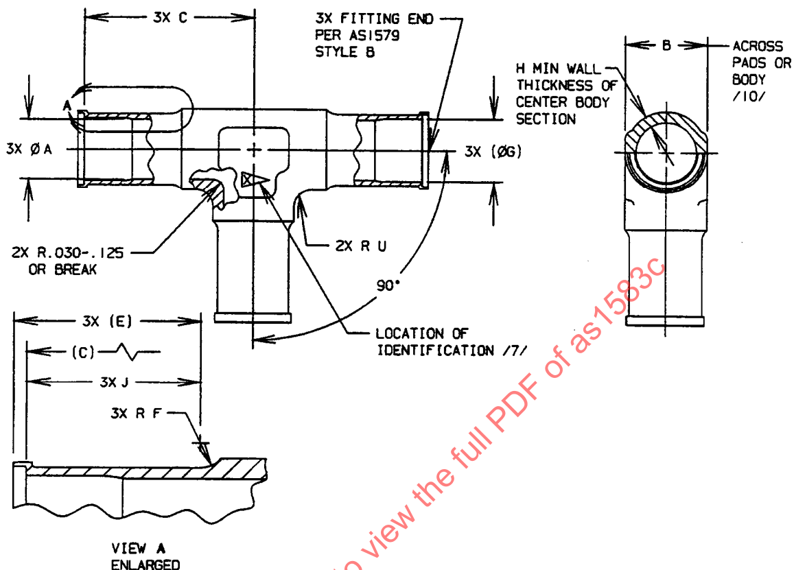
FIGURE 1 - FITTING, TEE
