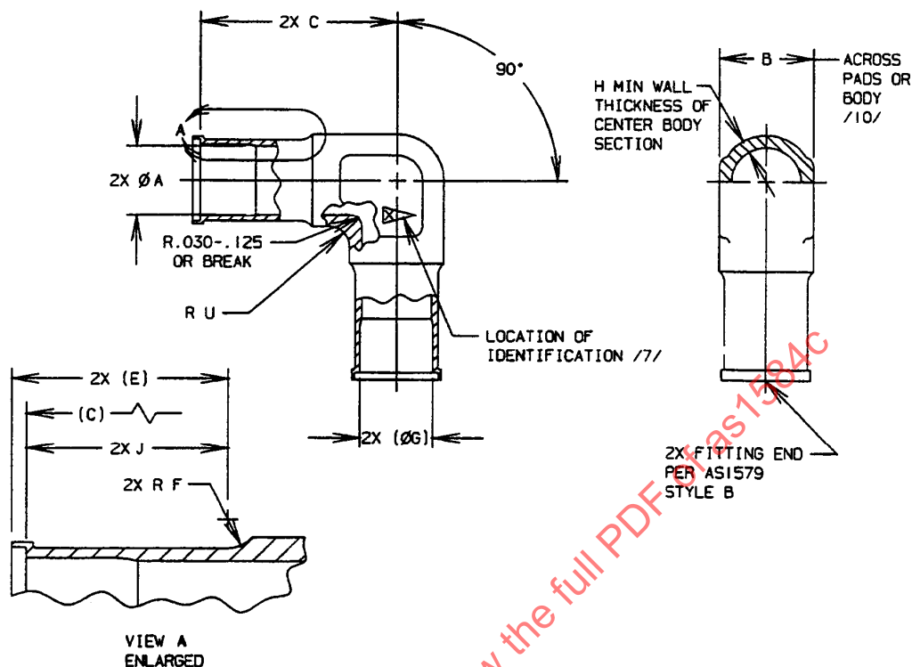
FIGURE 1 - FITTING, ELBOW, 90°
