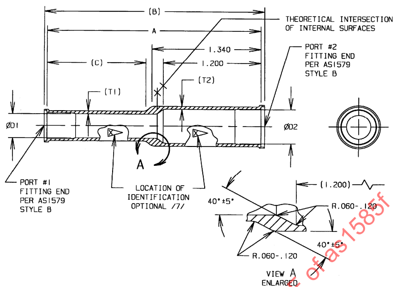
FIGURE 1 - FITTING, WELD RING
