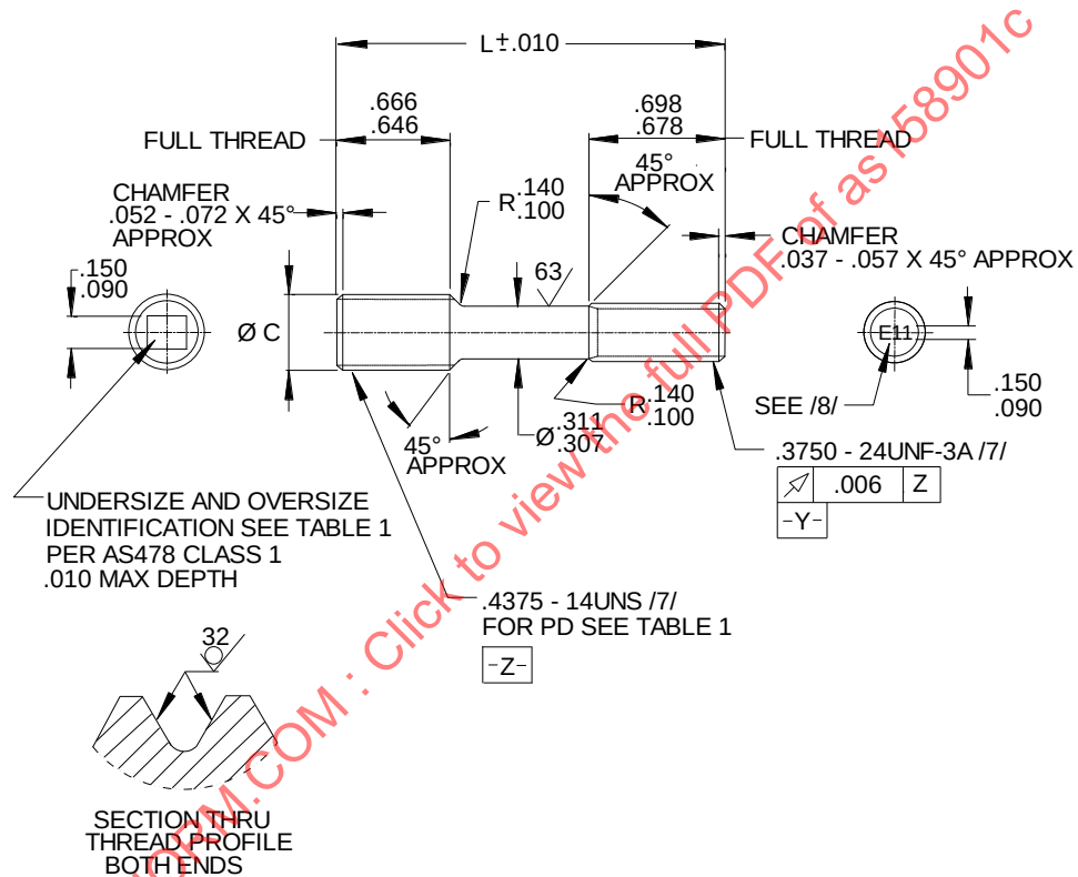
FIGURE 1 - STUD
