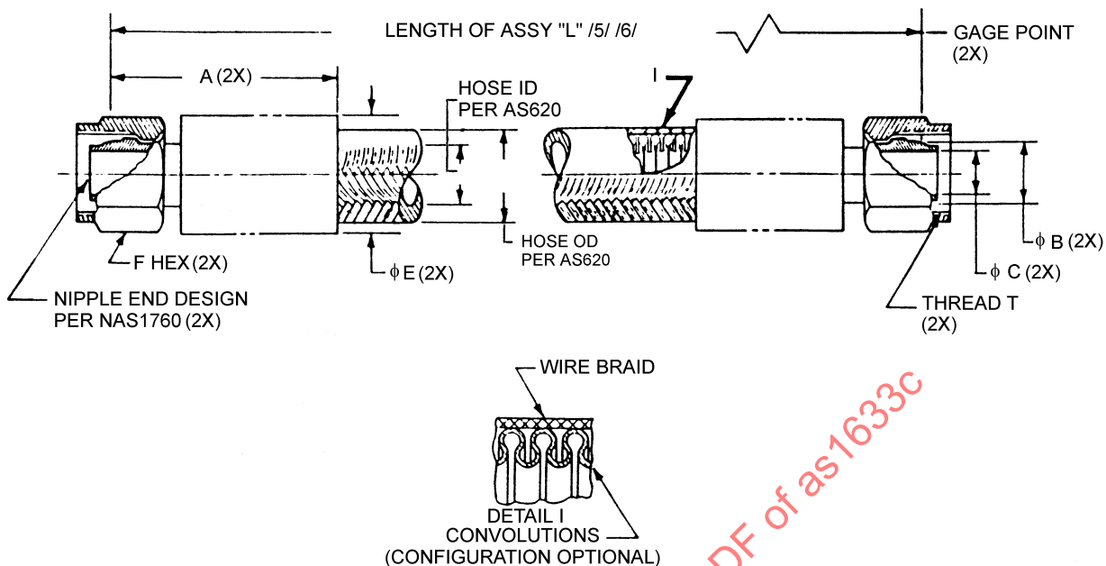
FIGURE 1 - HOSE ASSEMBLY
