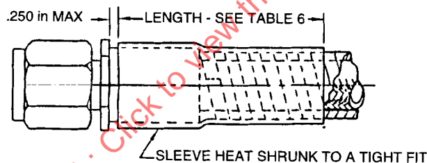
FIGURE 2 - SPIRAL ABRASION COVER /7/
