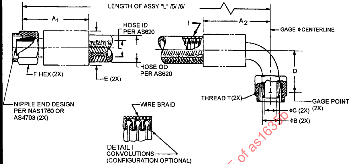
FIGURE 1 - HOSE ASSEMBLY
