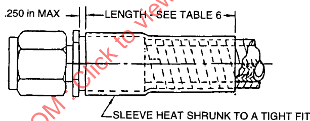
FIGURE 2 - SPIRAL ABRASION COVER /7/
