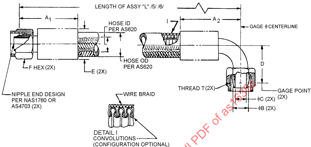
FIGURE 1 - HOSE ASSEMBLY
