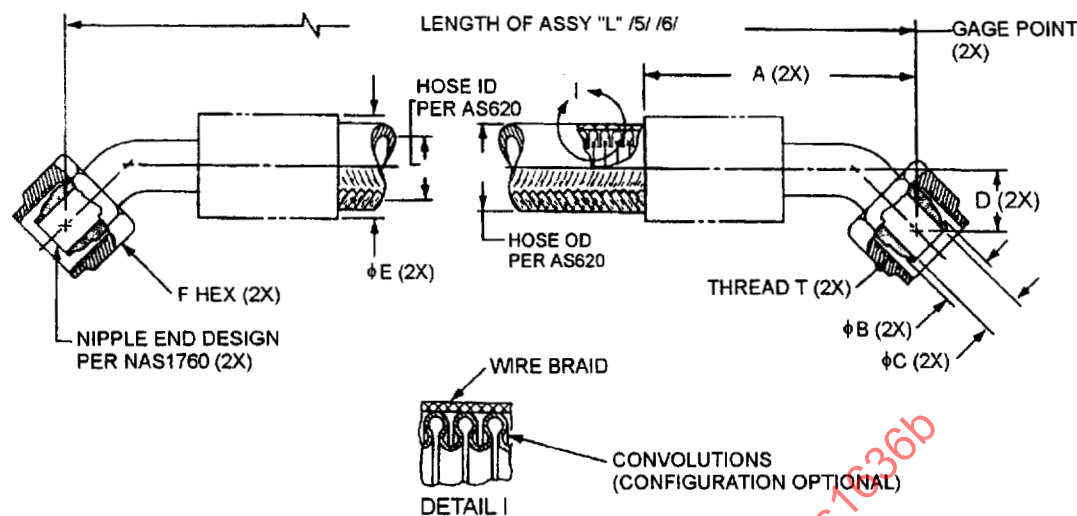
FIGURE 1 - HOSE ASSEMBLY
