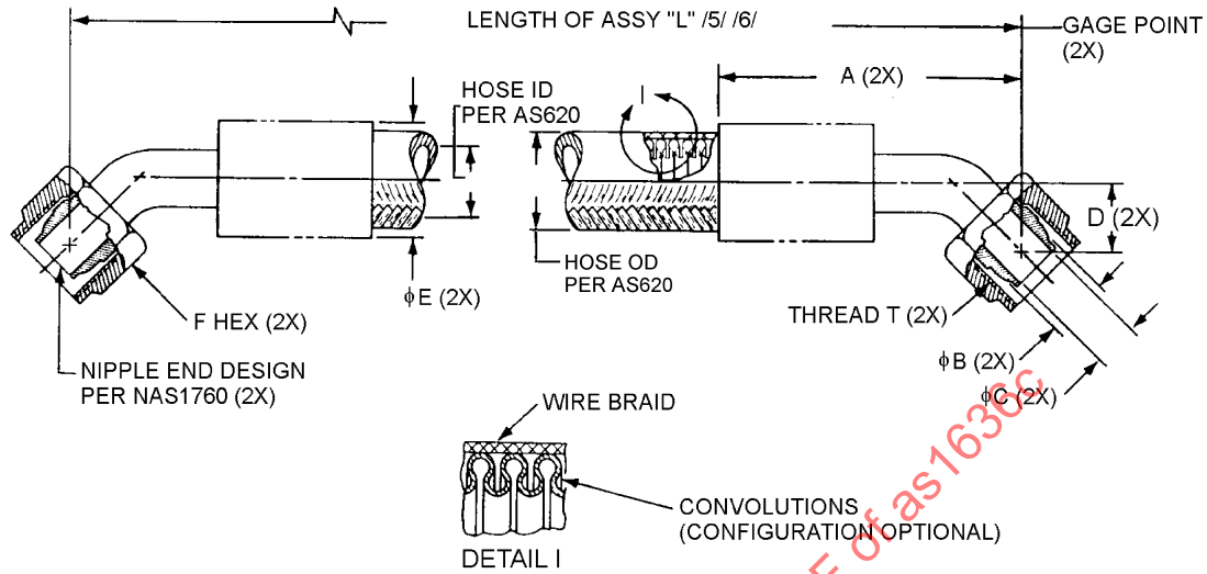
FIGURE 1 - HOSE ASSEMBLY
