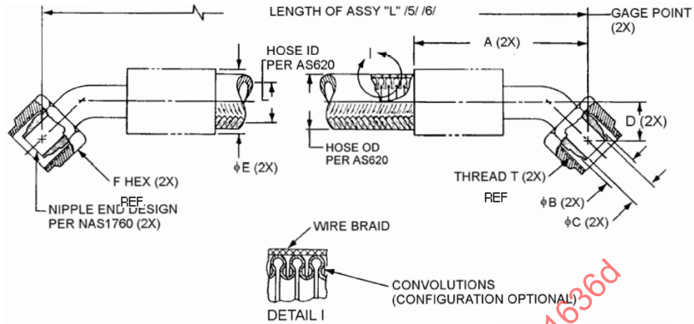
FIGURE 1 - HOSE ASSEMBLY
