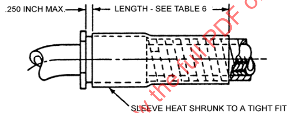
FIGURE 2 - SPIRAL AND POLYESTER ABRASION COVER /7/, /8/
