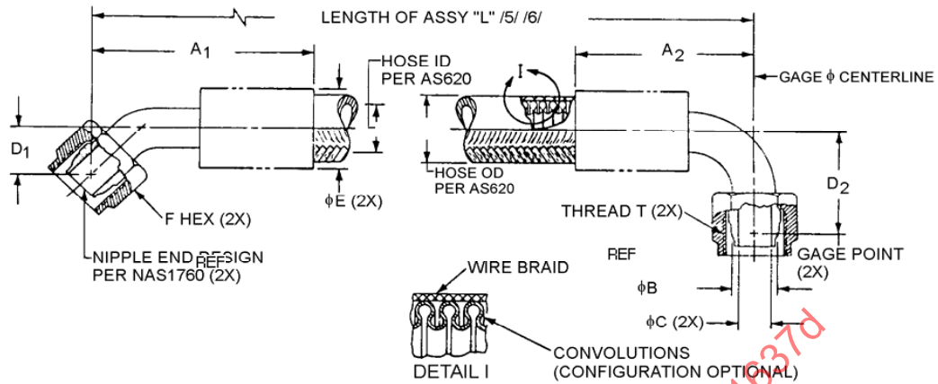
FIGURE 1 - HOSE ASSEMBLY
