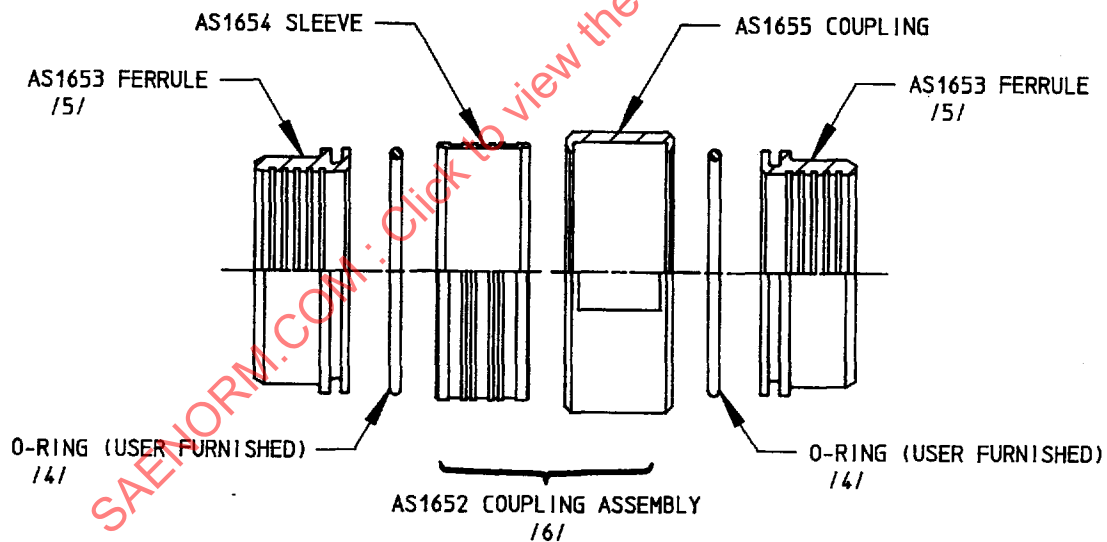
FIGURE 2 - EXPLODED VIEW OF COUPLING
