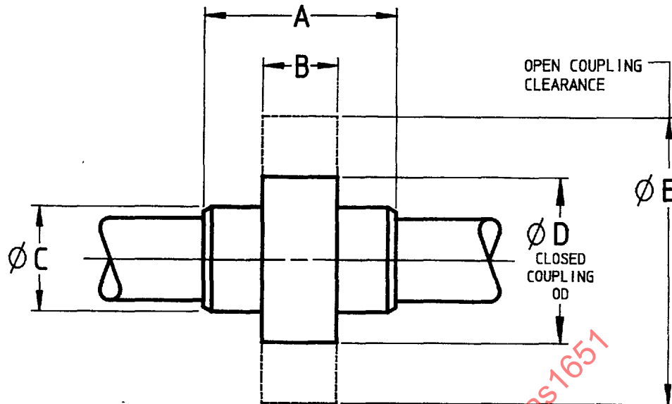
FIGURE 1 - ASSEMBLED COUPLING ENVELOPE
