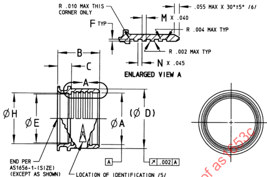
FIGURE 1 - MALE FERRULE
