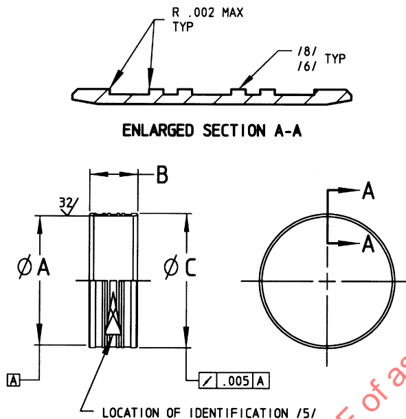
FIGURE 1 - SLEEVE
