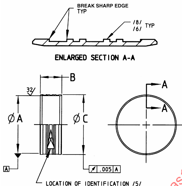
FIGURE 1 - SLEEVE
