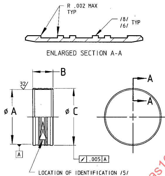
FIGURE 1 - SLEEVE
