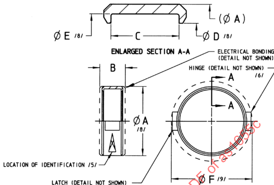
FIGURE 1 - COUPLING BODY
