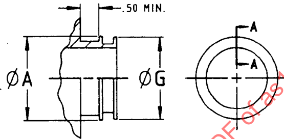
FIGURE 1 - FERRULE END
