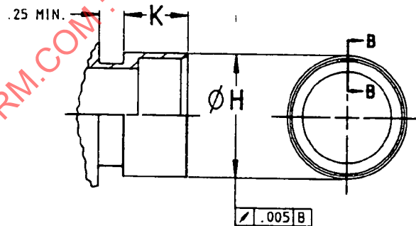
FIGURE 2 - SLEEVE END
