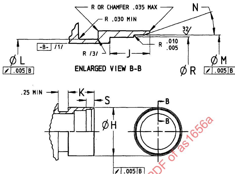
FIGURE 3 - SLEEVE END (FOR HOSE ENDS ONLY)
