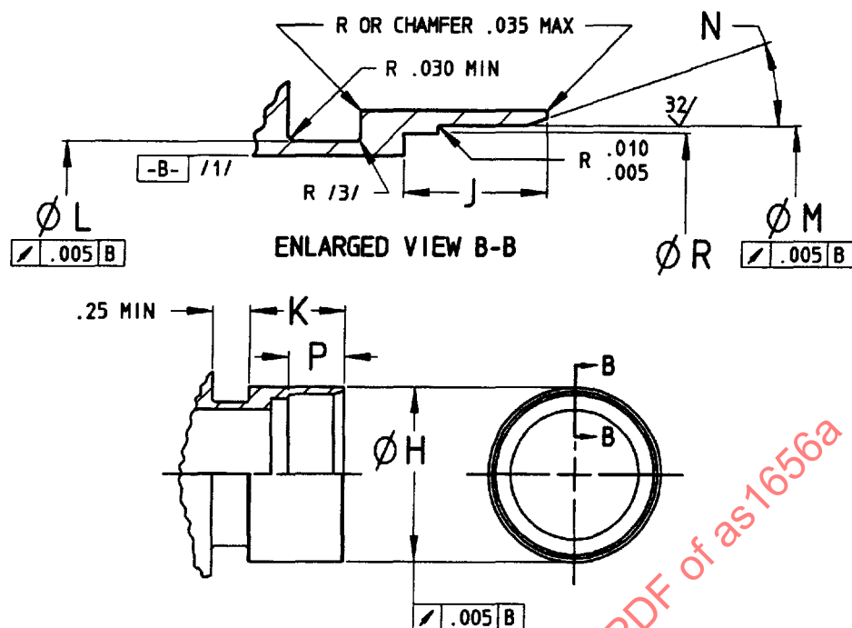
(R) FIGURE 2 - SLEEVE END
