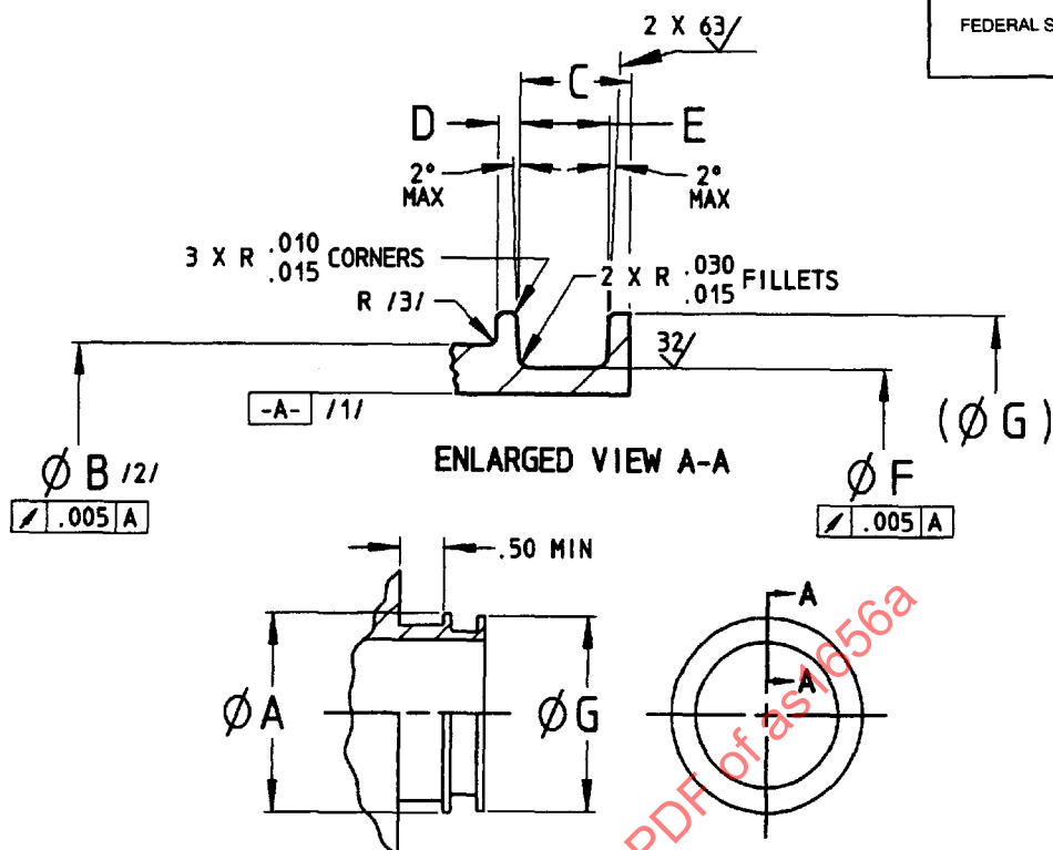
(R) FIGURE 1 - FERRULE END
