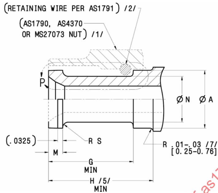
FIGURE 3 - FITTING END DESIGN, STYLE C SAME AS STYLE A EXCEPT AS SHOWN
