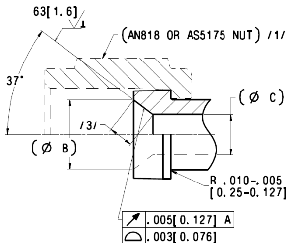
FIGURE 4 - FITTING END DESIGN, STYLE D /1/ SAME AS STYLE A EXCEPT AS SHOWN
