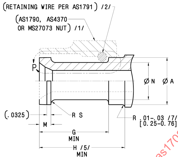
FIGURE 3 - FITTING END DESIGN, STYLE C SAME AS STYLE A EXCEPT AS SHOWN
