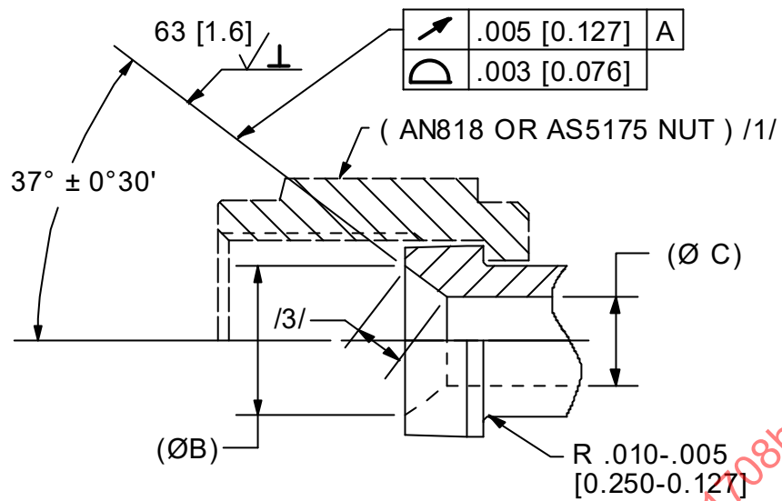
FIGURE 4 - FITTING END DESIGN, STYLE D /11/ SAME AS STYLE A EXCEPT AS SHOWN
