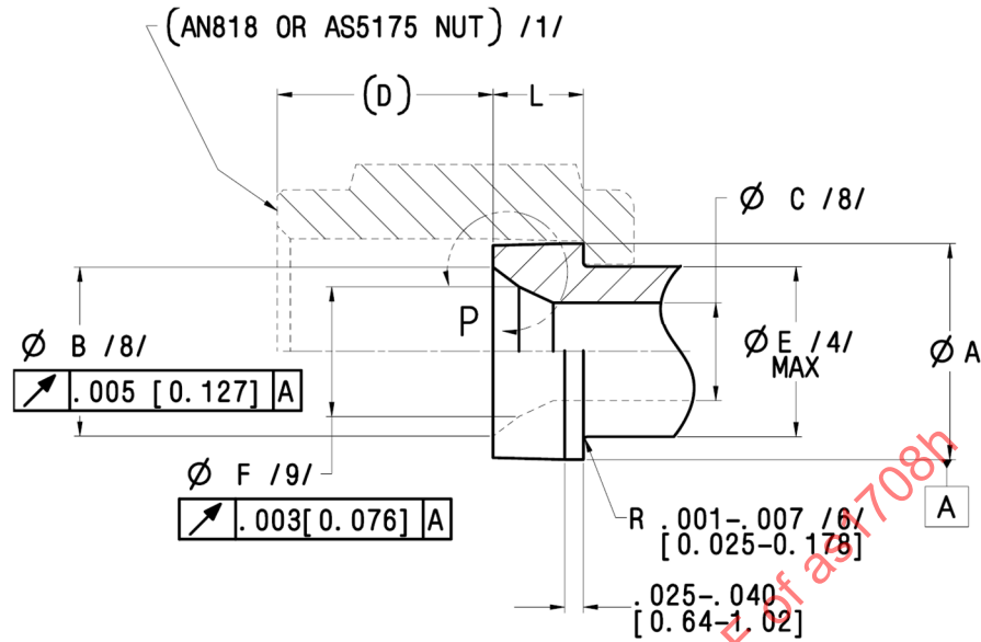
FIGURE 1 - FITTING END DESIGN, STYLE A
