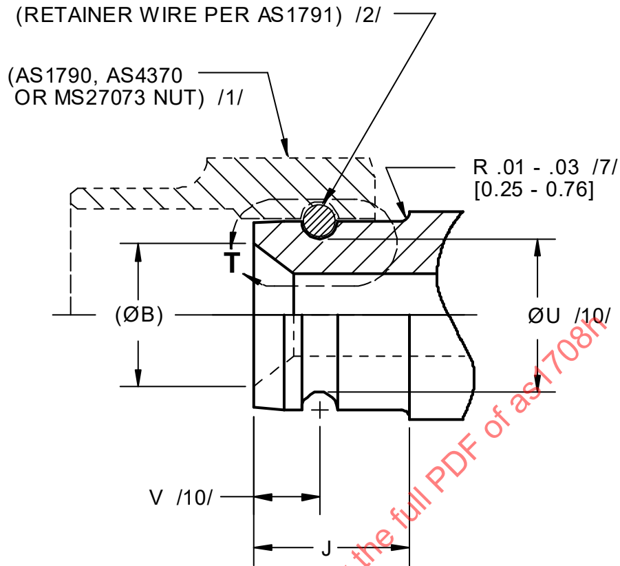
FIGURE 5 - FITTING END DESIGN, STYLE E /11/ SAME AS STYLE D EXCEPT AS SHOWN
