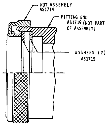
AS1713 HALF COUPLING SUB-ASSEMBLY
