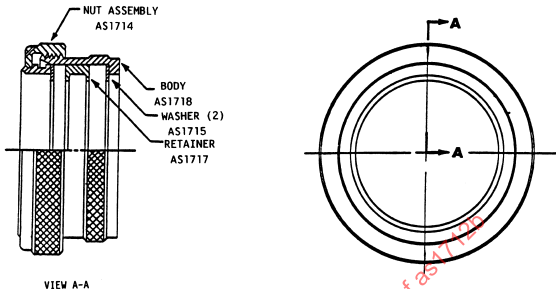
FIGURE 1 - COUPLING SUBASSEMBLY, FLEXIBLE
