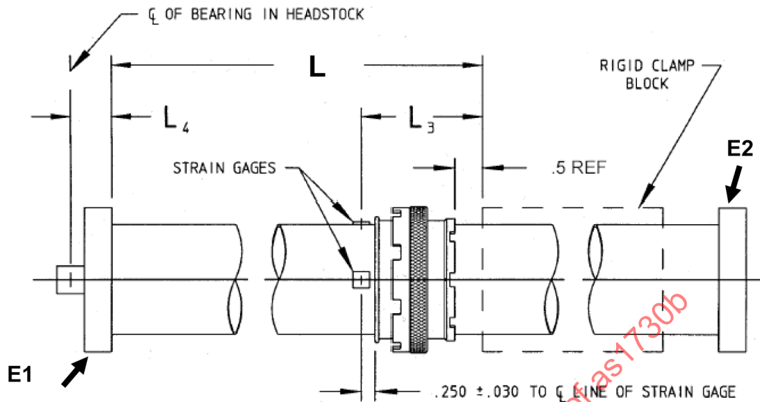
FIGURE 2 - FLEXURE TEST SPECIMEN CONFIGURATION
