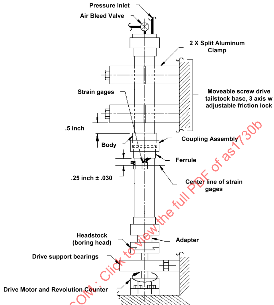
FIGURE 3 - TYPICAL ROTARY FLEXURE TEST SCHEMATIC
