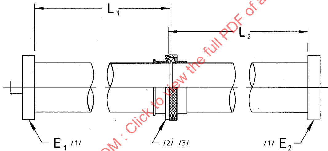
FIGURE 1 - TEST SPECIMEN CONFIGURATION
