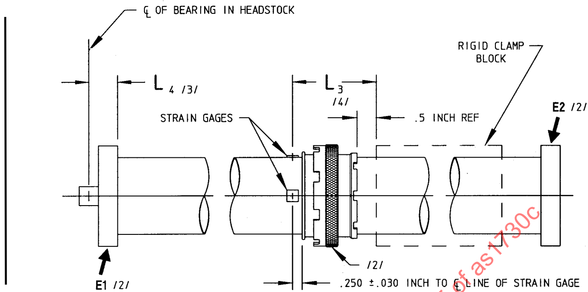
FIGURE 2 - FLEXURE TEST SPECIMEN CONFIGURATION
