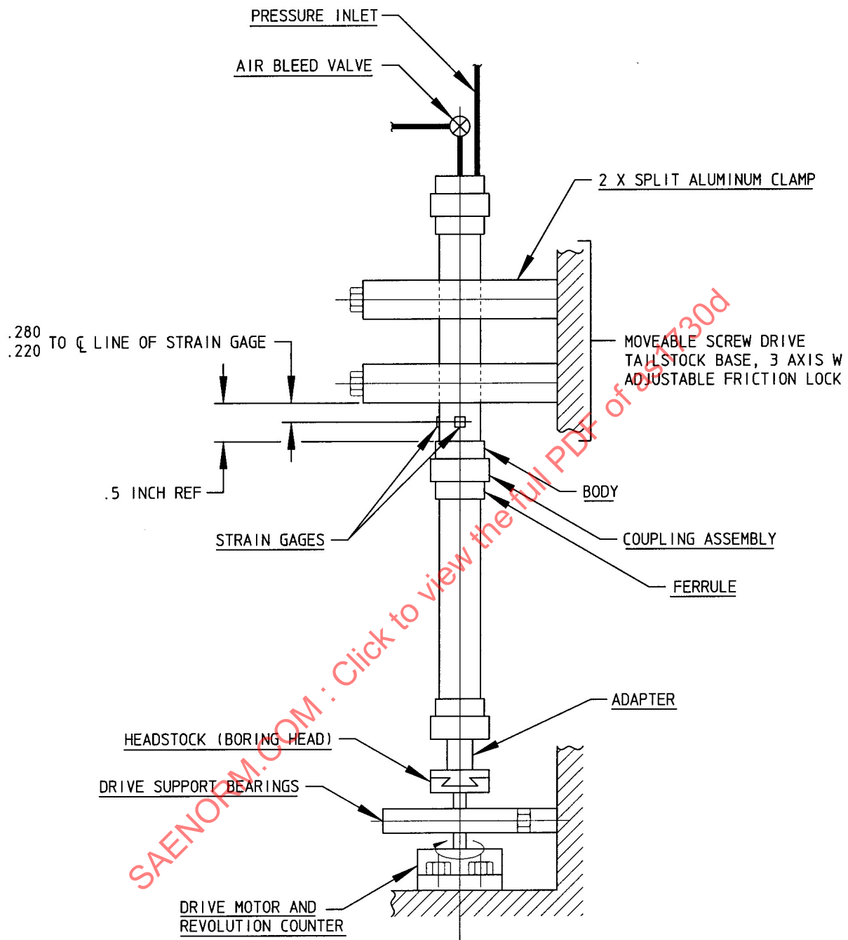
FIGURE 3 - TYPICAL ROTARY FLEXURE TEST SCHEMATIC
