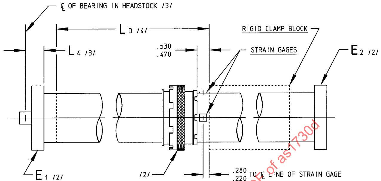
FIGURE 2 - FLEXURE TEST SPECIMEN CONFIGURATION
