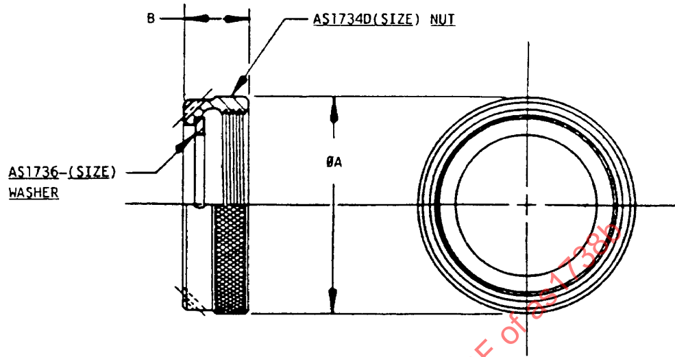
FIGURE 1 - TYPE I COUPLING NUT ASSEMBLY
