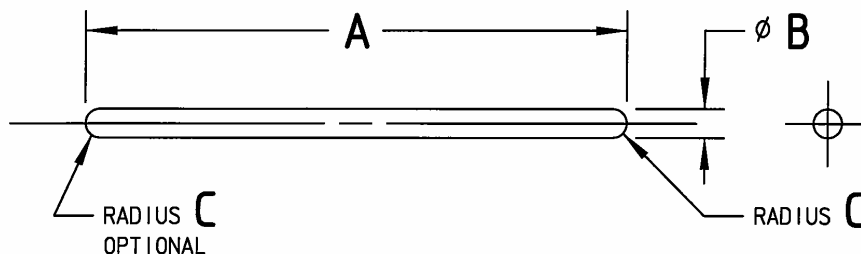
FIGURE 1 - WIRE, RETAINER
